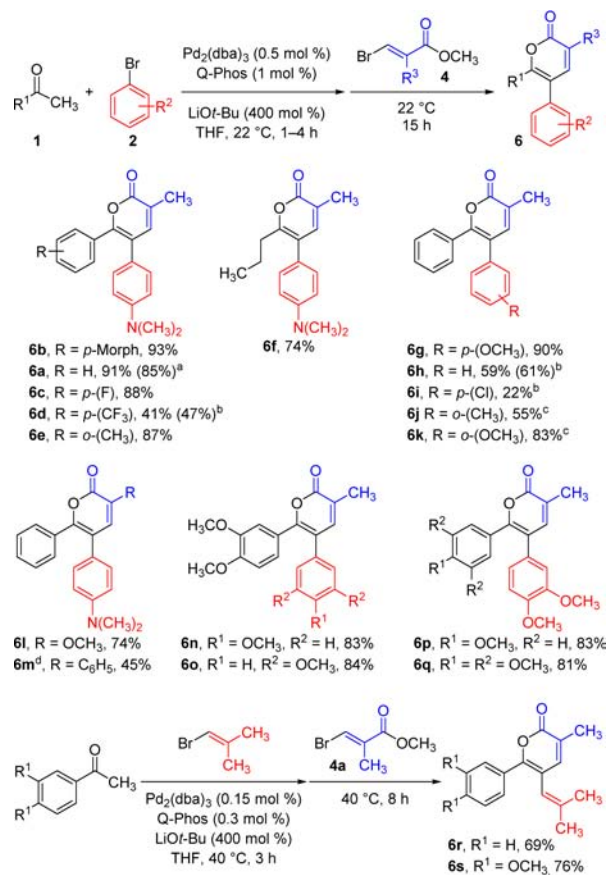
Figure 3. Investigation of the three-component synthesis of \alpha -pyrones using methyl ketones with aryl or alkenyl bromides and bromoacrylates. Reactions were conducted on a 0.5 mmol scale. Isolated yields are reported. a Conducted on a 4.5 mmol scale. b The second part of the sequence was conducted at 40 °C. c The entire reaction sequence was conducted at 40 °C. d The corresponding ethyl acrylate was employed.
