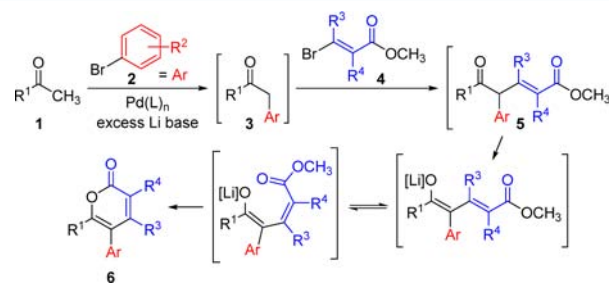
Figure 1. Proposed multicomponent pathway to \alpha -pyrones.
