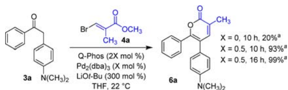
Figure 2. Examination of reaction conditions for the combination of \alpha -alkenylation and subsequent isomerization/lactonization. a Yield based on NMR internal standard.
